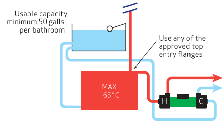
Figure 24: Horizontal cylinders
