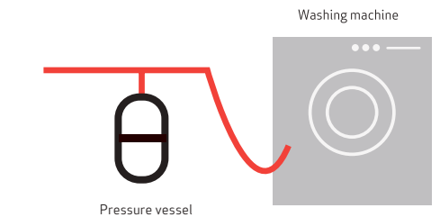
Figure 28: Water hammer protection
