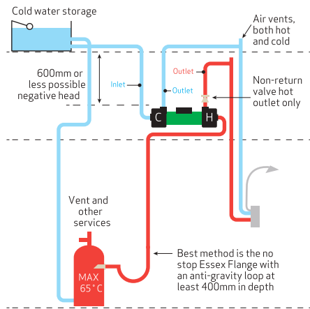
Figure 22: Anti-gravity loop (AGL)
