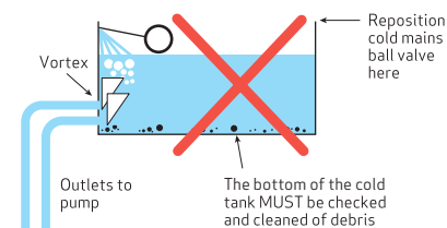
Figure 16: Aeration
