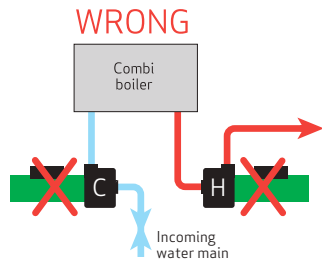
Figure 23: Combi boilers
