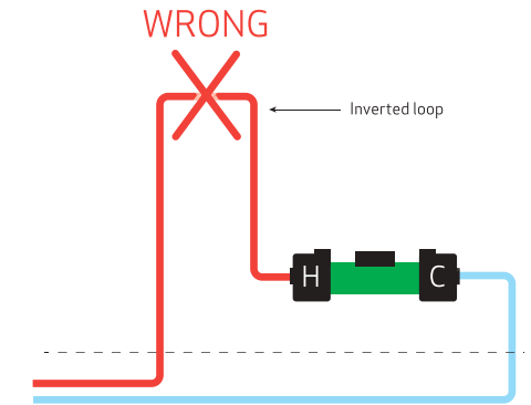
Figure 27: Inverted loops
