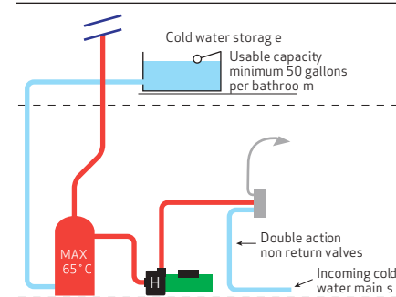
Figure 13: Tank fed (hot) with mains cold
