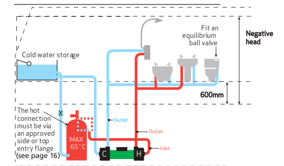
Figure 9: Negative head
